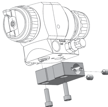
Option 1. 12.7mm Mounting hole
