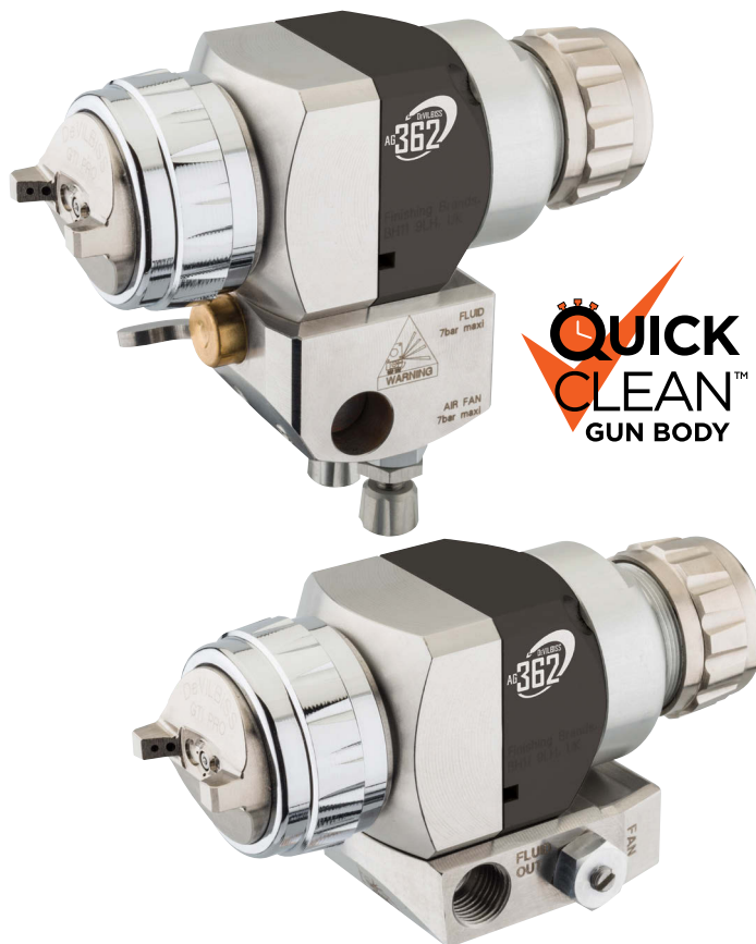
Shown above Right AG362-TE40-085N-S Left AG362-C3-14-L
