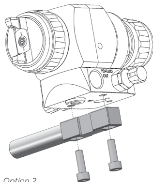
Option 2. 12.7mm x 60mm long Mounting Bar
